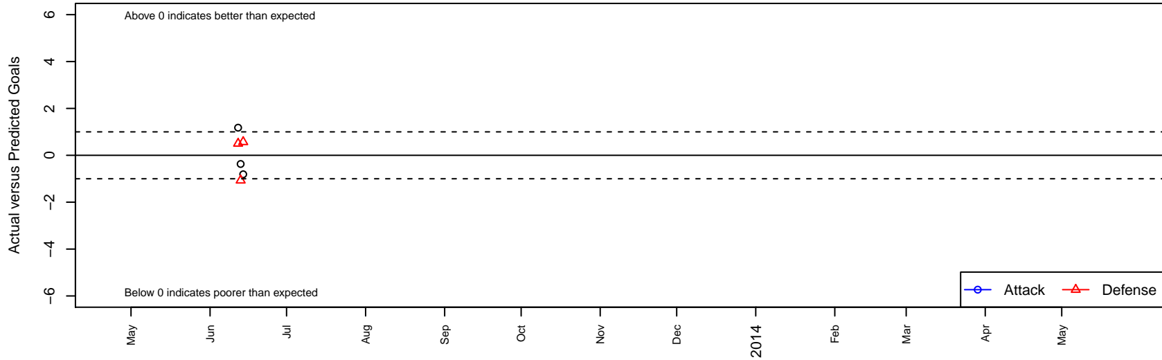
Alaska Rush G99 Dots are actual minus expected GF (blue circles) and GA (red triangles). Blue line is smoothed change in attack strength. Red is smoothed change in defense strength.
